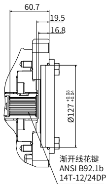
“CC”型通轴驱动
