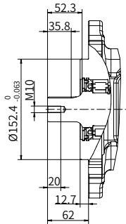
“D0” 型花键轴 ANSI B92.1b 1 1/2 in 23T 16/32 DP
