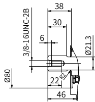
“B3” 型花键轴 ANSI B92.1b 1 in 15T 16/32DP
