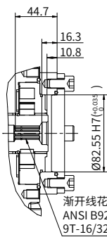
“A1”型通轴驱动
