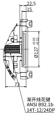
“CC”型通轴驱动
