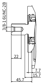
“B3” 型花键轴 ANSI B92.1b 1 in 15T 16/32DP
